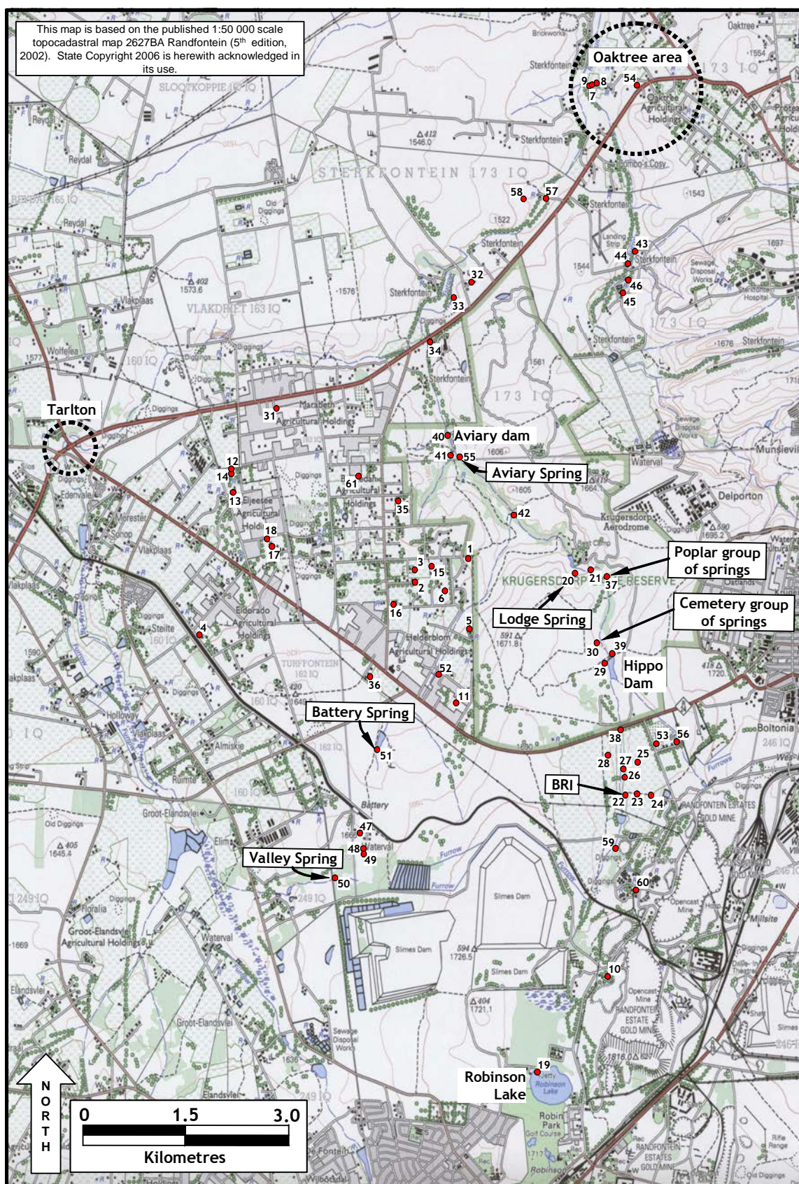
Figure 8. Geosite locality map
