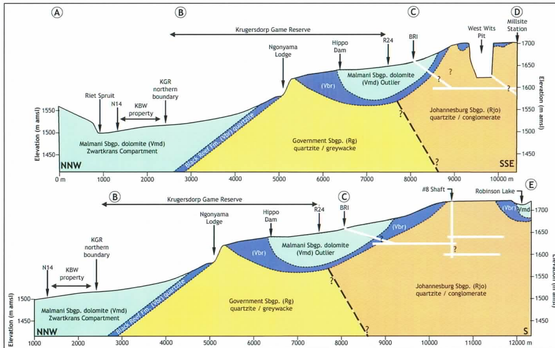
Figure 5a. Conceptual geologic profiles (see Figure 4 for profile positions)
