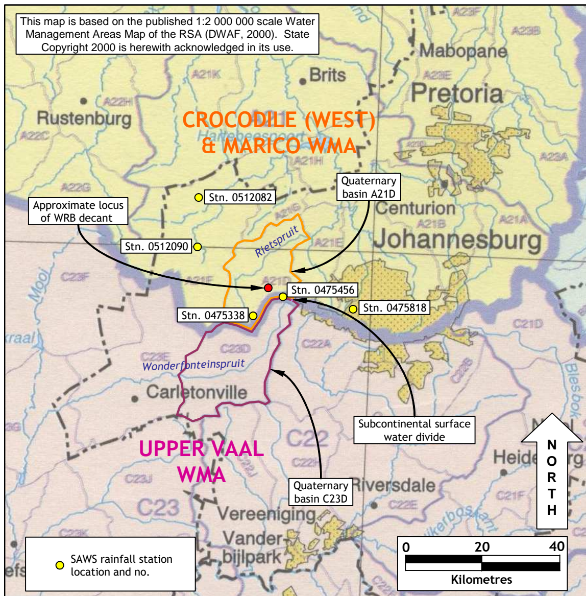
Figure 2. Regional surface water drainage map
